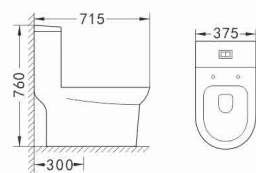
R022 Siphonic One Piece Toilet Size: 715 × 375 × 760mm S-trap, 300mm Roughing-in
