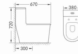
R230 Siphonic One Piece Toilet Size: 670 × 380 × 720mm S-trap, 300mm Roughing-in
