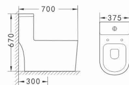
R150 Siphonic One Piece Toilet Size: 700 × 375 × 670mm S-trap, 300mm Roughing-in
