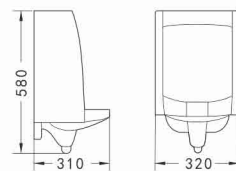
UR602 Outlet Wall-hung Urinal Size: 320 × 310 × 580mm Top / Back inlet & Back/ Bottom outlet
