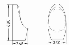
UR605 Wall-hung Urinal Size: 330 × 265 × 680mm Top Inlet & Bottom Outlet
