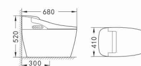
R2014B Foot Touch Flushing R2014C Automatic Cover All-in-one Toilet Size: 680 × 410 × 520mm S-trap:250,300 mm roughing-in P-trap:180 mm roughing-in Siphonic flushing
