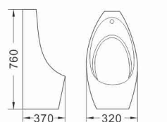
UR672 Wall-hung Urinal Size: 320 × 370 × 760mm Back inlet & Back Outlet
