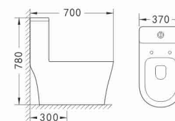
R206 Siphonic One Piece Toilet Size: 700 × 370 × 780mm S-trap, 300mm Roughing-in
