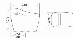
R2208B Foot Touch Flushing R2208C Automatic Cover All-in-one Toilet Size: 680 × 420 × 520mm S-trap:250,300 mm roughing-in P-trap:180 mm roughing-in Siphonic flushing
