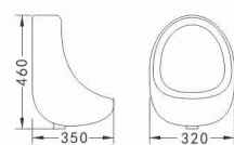
UR608 Wall-hung Urinal Size: 320 × 350 × 460mm Top Inlet & Bottom Outlet
