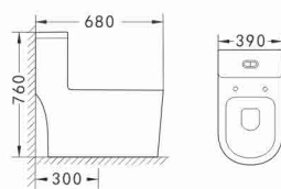
R149 Siphonic One Piece Toilet Size: 680 × 390 × 760mm S-trap, 300mm Roughing-in
