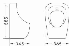
UR310 Wall-hung Urinal Size: 365 × 345 × 585mm Top / Back inlet & Back Outlet
