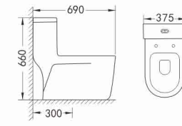
R228 Siphonic One Piece Toilet Size: 690 × 375 × 660mm S-trap, 300mm Roughing-in
