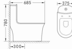
R239 Siphonic One Piece Toilet Size: 685 × 375 × 780mm S-trap, 300mm Roughing-in Vortex Flush
