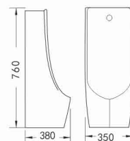
UR632 Wall-hung Urinal Size: 350 × 380 × 760mm Top / Back Inlet & Back Outlet
