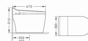
R2209B Foot Touch Flushing R2209C Automatic Cover All-in-one Toilet Size: 670 × 380 × 510mm S-trap:300,400 mm roughing-in P-trap:180 mm roughing-in Siphonic flushing
