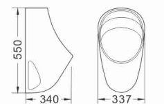
UR628 Wall-hung Urinal Size: 337 × 340 × 550mm Back Inlet & Back Outlet
