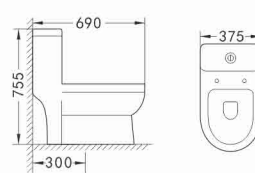
R023 Siphonic One Piece Toilet Size: 690 × 375 × 755mm S-trap, 300mm Roughing-in
