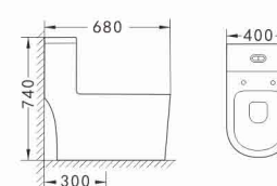
R248 Siphonic One Piece Toilet Size: 680 × 400 × 740mm S-trap, 300mm Roughing-in Vortex Flush
