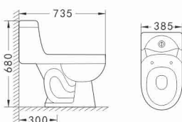
R028 Siphonic One Piece Toilet Size: 735 × 385 × 680mm S-trap, 300mm Roughing-in
