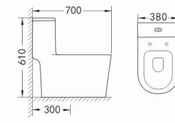
R231 Siphonic One Piece Toilet Size: 700 × 380 × 610mm S-trap, 300mm Roughing-in
