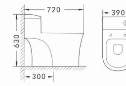
R208 Siphonic One Piece Toilet Size: 720 × 390 × 630mm S-trap, 300mm Roughing-in
