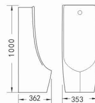
UR633 Stand Urinal Size: 353 × 362 × 1000mm Top / Back Inlet & Back Outlet
