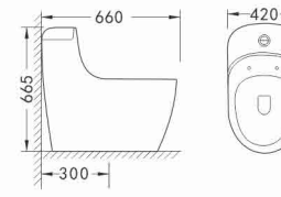
R232 Siphonic One Piece Toilet Size: 660 × 420 × 665mm S-trap, 300mm Roughing-in
